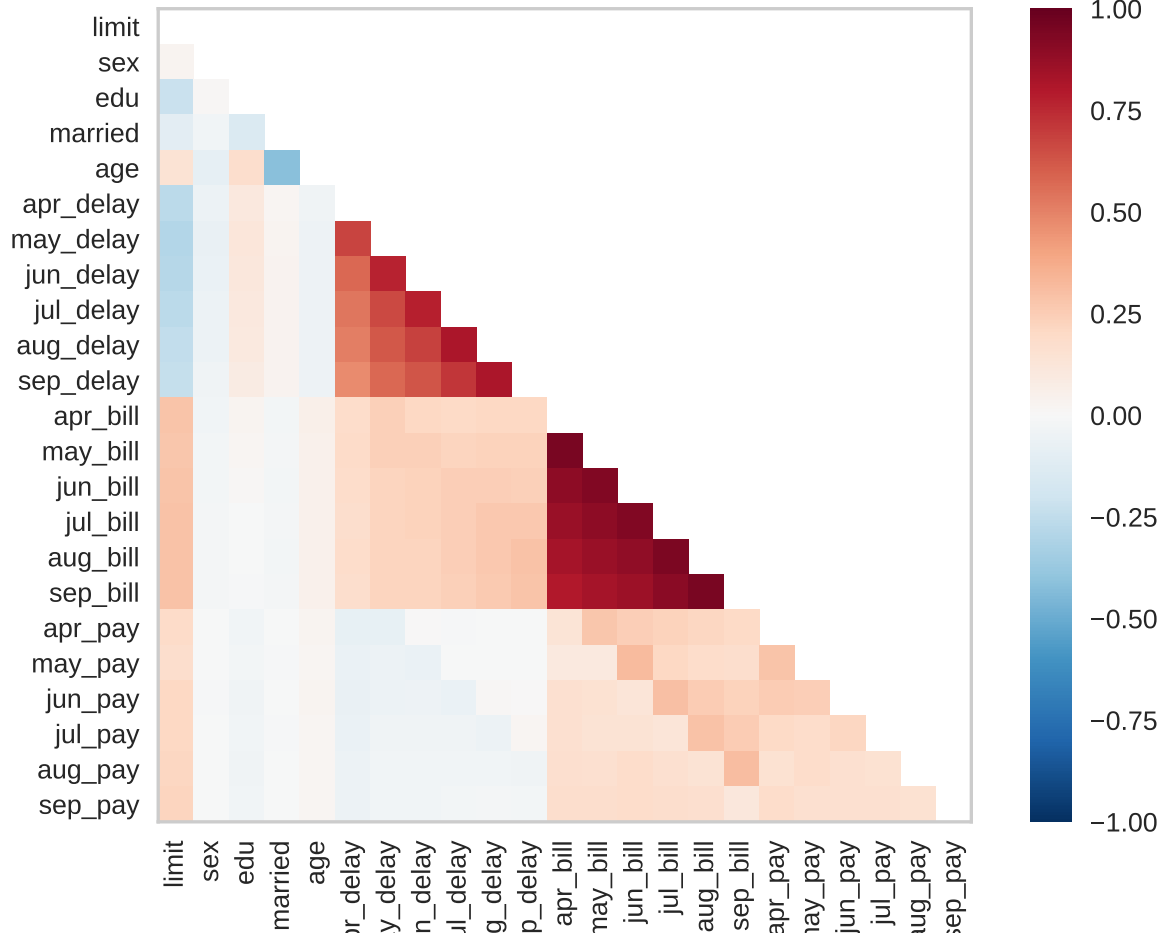
Pearson Ranking of 23 Features
