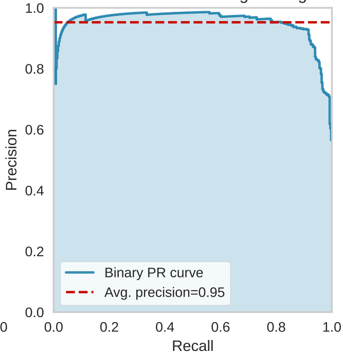
Precision-Recall Curve for LogisticRegression
