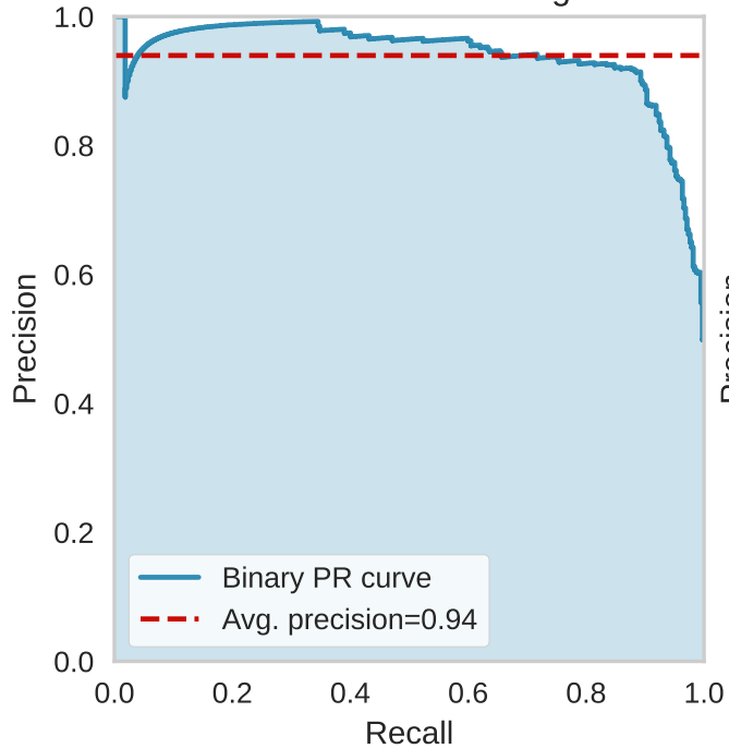
Precision-Recall Curve for RidgeClassifier
